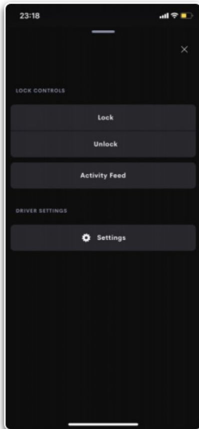
User Screen
