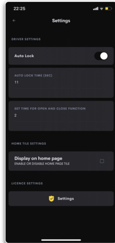
Settings Page
